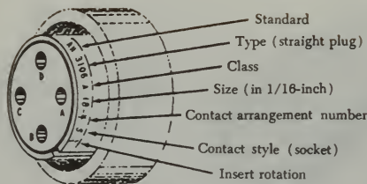
FIGURE 4-119. AN connector marking.
